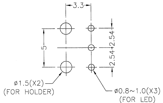
MOUNTING HOLE
