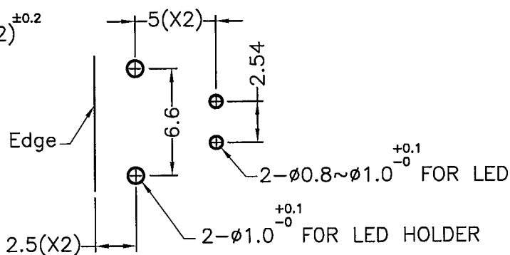
RECOMMEND MOUNTING HOLES
