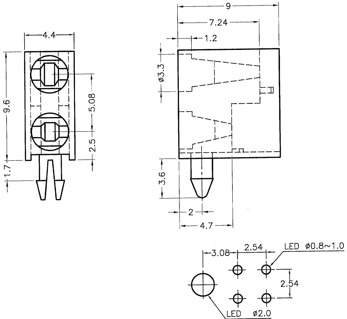
MOUNTING HOLES
