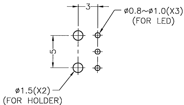
MOUNTING HOLE
