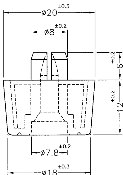
BODY
