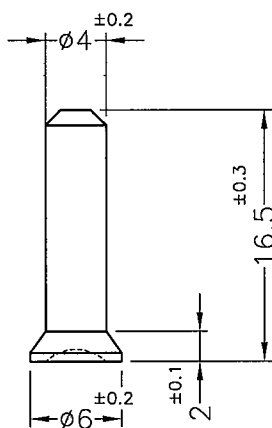
PIN
