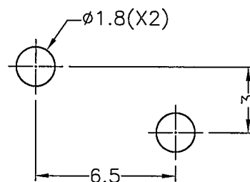
HOUNTING HOLE
