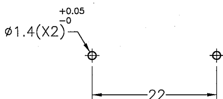
MOUNTING HOLE (RECOMMEND FOR REFERENCE ONLY)
