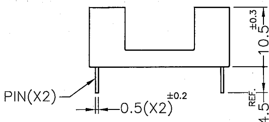
FUSE HOLDER
