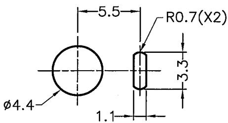
MOUNTING HOLE
