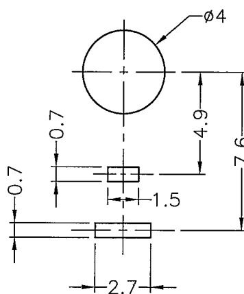
MOUNTING HOLE
