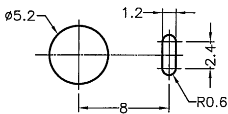
MOUNTING HOLE
