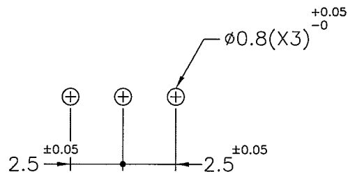
MOUNTING HOLE
