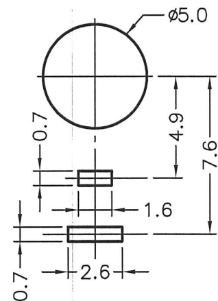
MOUNTING HOLE
