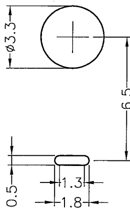
MOUNTING HOLE
