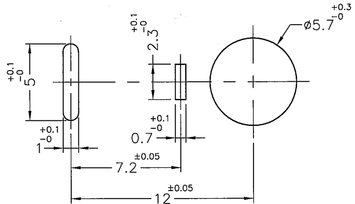
MOUNTING HOLE
