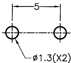
MOUNTING HOLE
