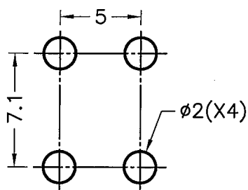
MOUNTING HOLE
