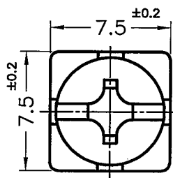
(SCREW)PCB-10B
