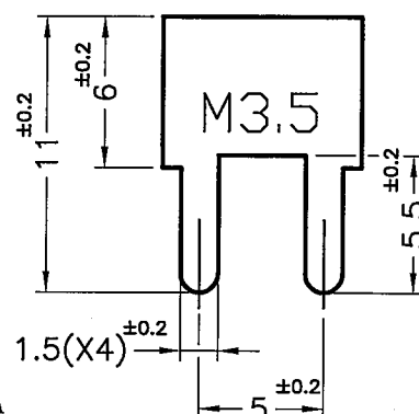
(BODY)PCB-10A
