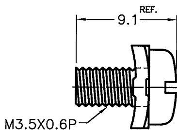
(SCREW)PCB-10B
