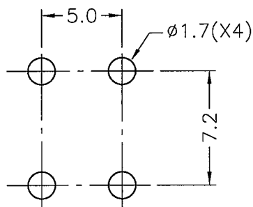
MOUNTING HOLE
