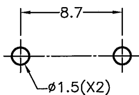
MOUNTING HOLE
