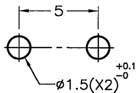
MOUNTING HOLE
