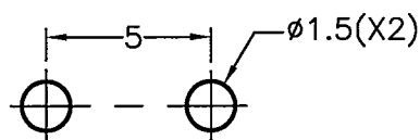
MOUNTING HOLE
