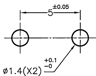
MOUNTING HOLE
