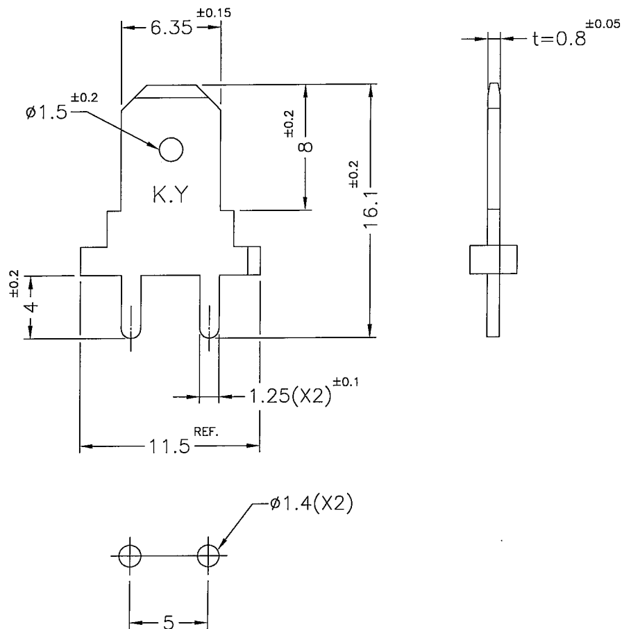
MOUNTING HOLE
