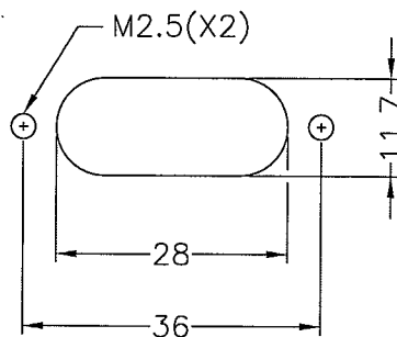
MOUNTING HOLE
