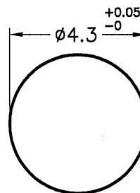
MOUNTING HOLE
