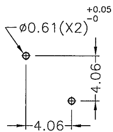
MOUNTING HOLE
