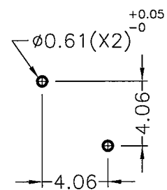
MOUNTING HOLE
