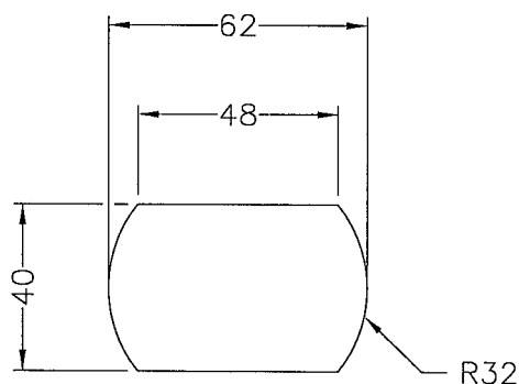
MOUNTING HOLE (RECOMMEND FOR REFERENCE ONLY)
