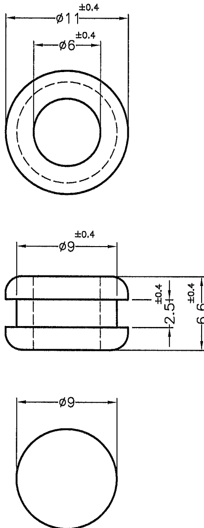
MOUNTING HOLES
