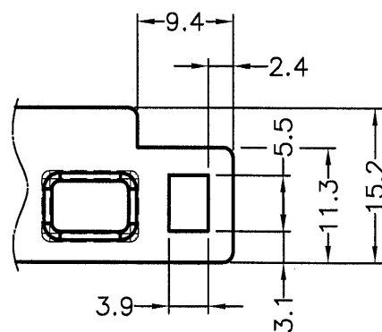
ASSEMBLY PART
