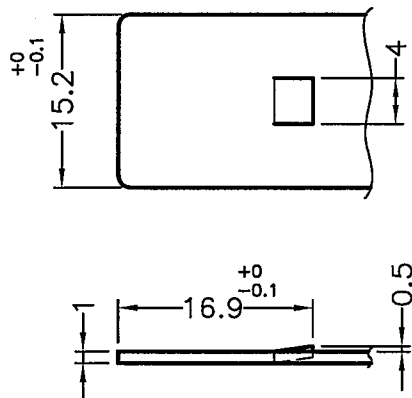
ASSEMBLY PART
