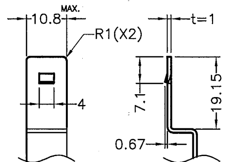
ASSEMBLY PART (裝配件尺寸, 僅供參考)
