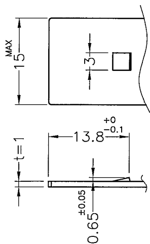
ASSEMBLY PART (裝配件尺寸, 僅供參考)
