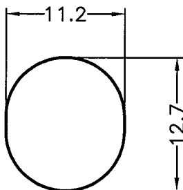
HOLE IN CHASSIS
