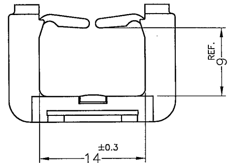
UNIT FOLDED VIEW (產品扣合示意圖)
