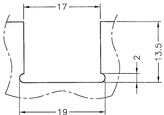
MOUNTING HOLE THICKNESS: 0.8~2.0mm (RECOMMEND FOR REFERENCE ONLY)
