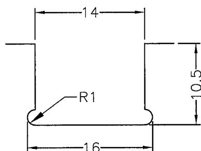
MOUNTING HOLE THICKNESS 0.8~2.0mm
