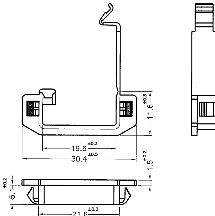
PANEL MOUNTING DETAILS
