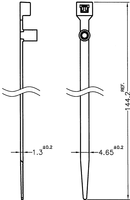
CABLE TIES
