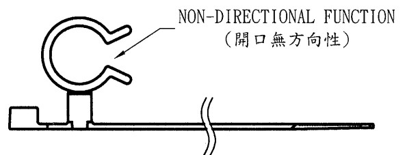
ASSEMBLING SCHEMATIC DIAGRAM 組裝示意圖
