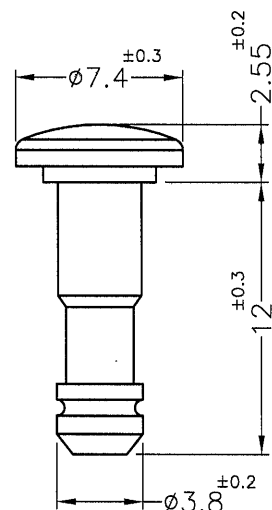
PIN
