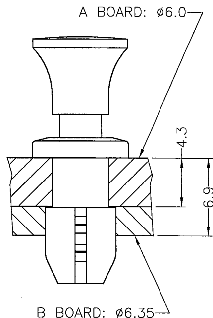
MOUNTING HOLE (RECOMMEND FOR REFERENCE ONLY)
