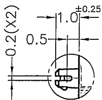
DETAIL C SCALE 6:1
