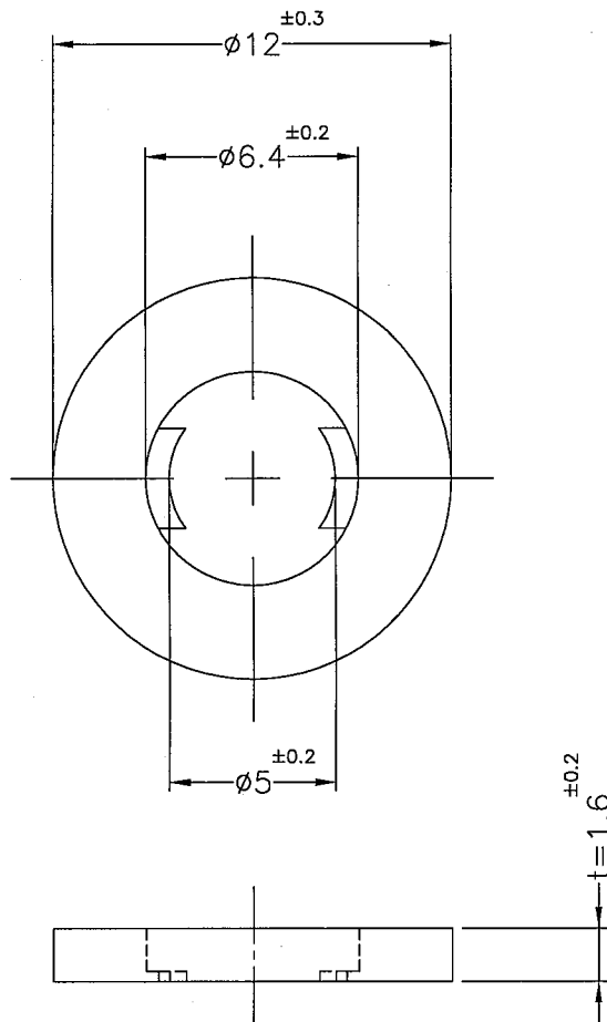
MATING SCREW M6 (RECOMMEND FOR REFERENCE ONLY)
