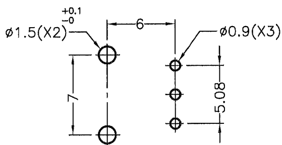
MOUNTING HOLES
