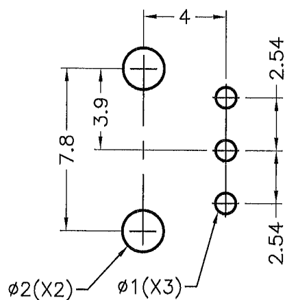
MOUNTING HOLES
