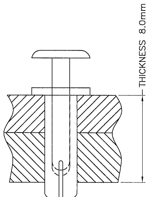
MOUNTING HOLE: \phi 3.5
