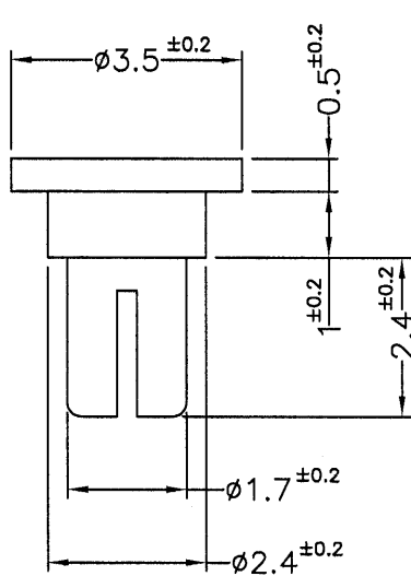
(BODY)
