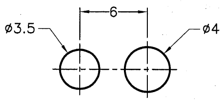
MOUNTING HOLES
