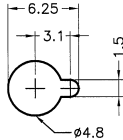
MOUNTING HOLE CHASSIS THICKNESS 1.6mm
