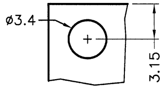
MOUNTING HOLE CHASSIS THICKNESS 1.2mm
