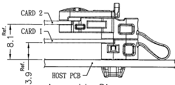
Assembly Diagram
