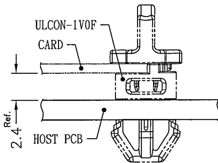
Assembly Diagram
