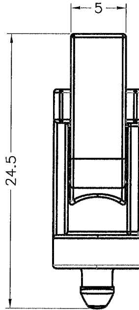
HOLE IN P.C.B P.C.B THICKNESS:1.57mm
