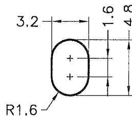
HOLE IN P.C.B P.C.B THICKNESS:1.57mm
